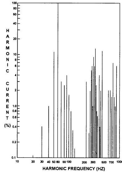
Figure 2 - Typical Cycloconverter Current Spectrum (60 Hz Power System)
